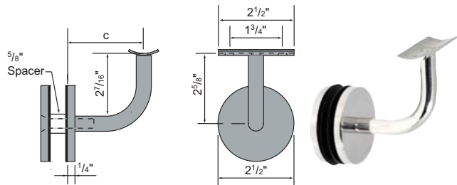
Supplied with M8 Countersunk, Phillips Head Bolt
